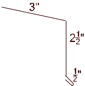
DENVER EAVE CE-1
