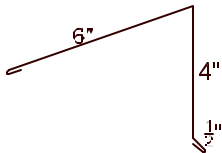
RIDGE/HIP FLASH RR-1
