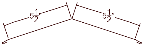
RESIDENTIAL RIDGE/HIP FLASH RR-1
