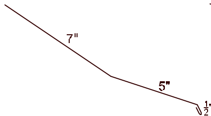
TRANSITION FLASH AT-1
