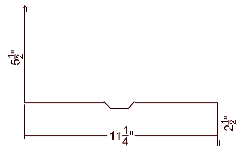
SOFFIT BOX - SOLID AB-3 WHITE VENTED AVAILABLE
