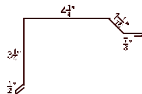
TRANSITION FLASH AT-1
