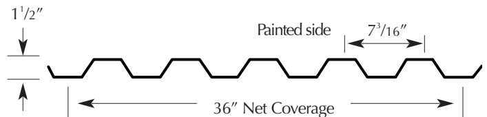
Reversed HR-36 Wall (typical wall applications)
