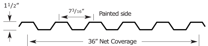
HR-36 Roof & Wall (Typical Roof Application)
