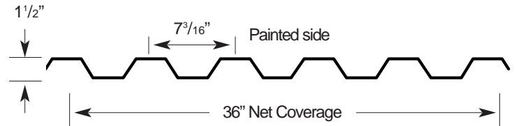
HR-36 Roof & Wall (Typical Roof Application)
