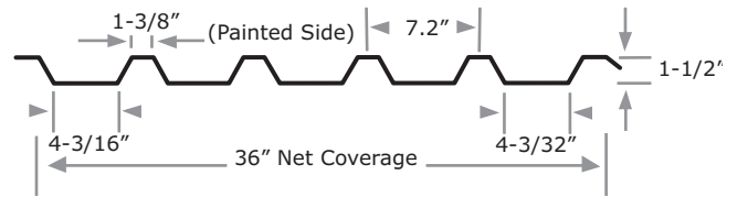
Reversed Box Rib (typical Roof and Wall applications)
