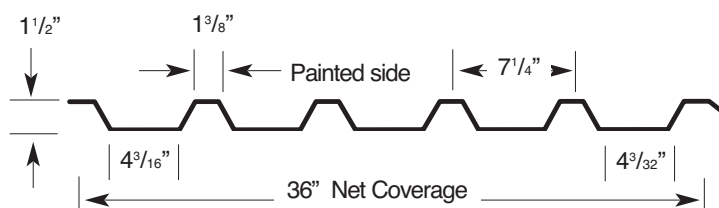
Reversed Box Rib (Typical Roof and Wall Panel)
