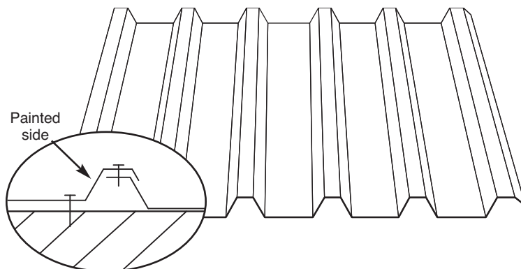
Lap Detail
